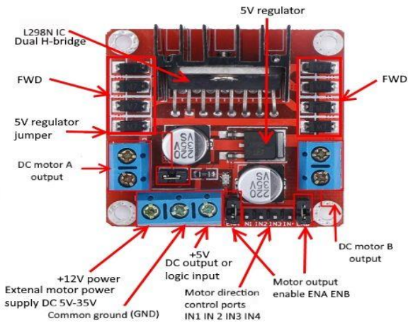
Figure 3. Motor Driver L298N
