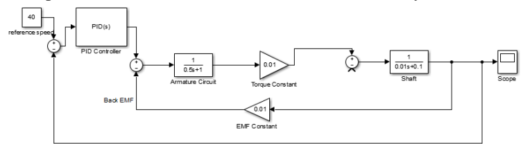
Figure 5. Simulation of the DC motor with controller
