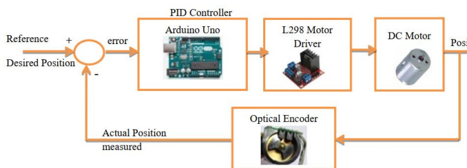
Figure 1. Block Diagram for DC Motor Speed Control
